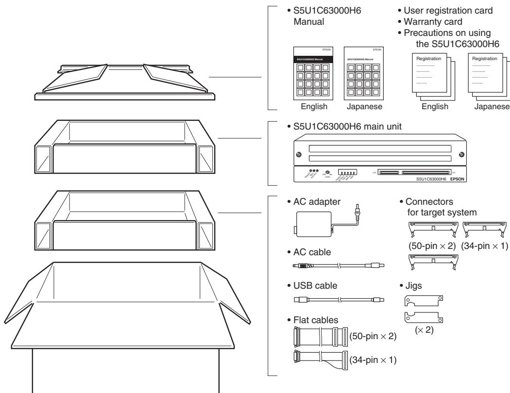
Figure 2.1.1 S5U1C63000H6 Package Structure
