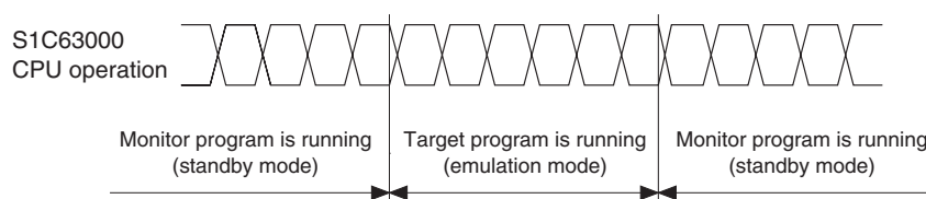
Figure 5.13.1 Operation of S1C63000 CPU
